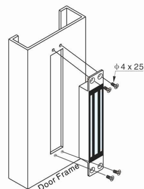
(4) Fix screws
