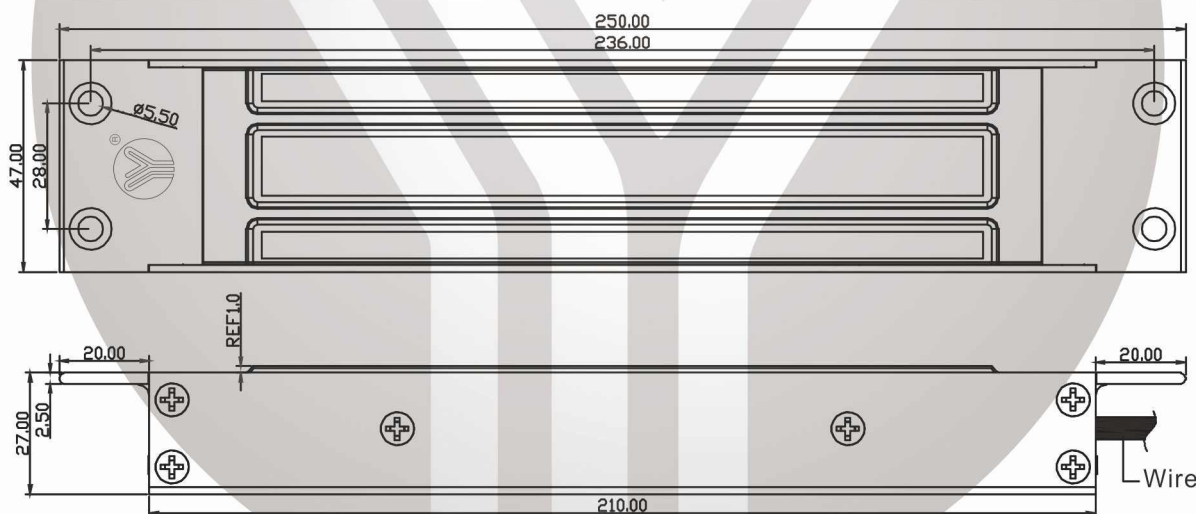
Magnetic Lock with Signal Output
