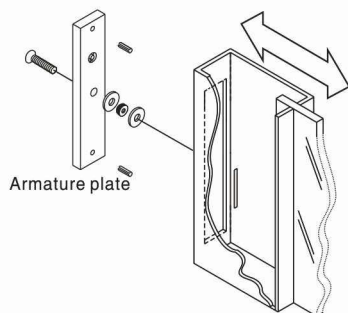
(2) Fix screws
